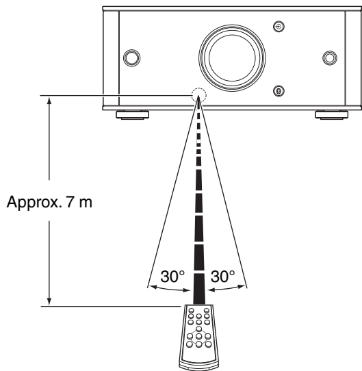
[Horizontal installation]
